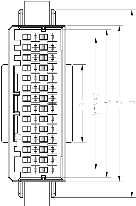
28POS(X-KEY): I-1903128-4
