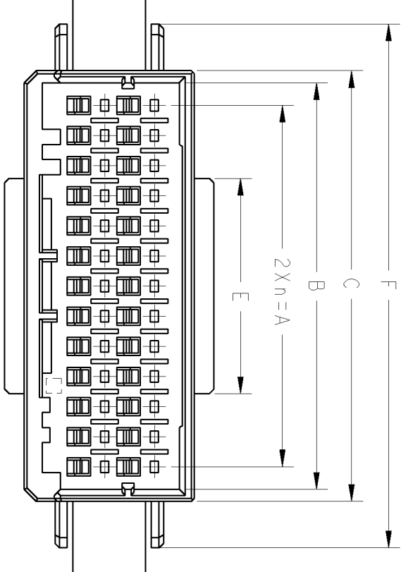
26POS(X-KEY): I-1903128-3
