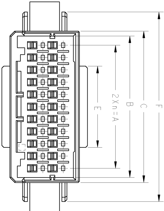
22POS(X-KEY): I-1903128-1
