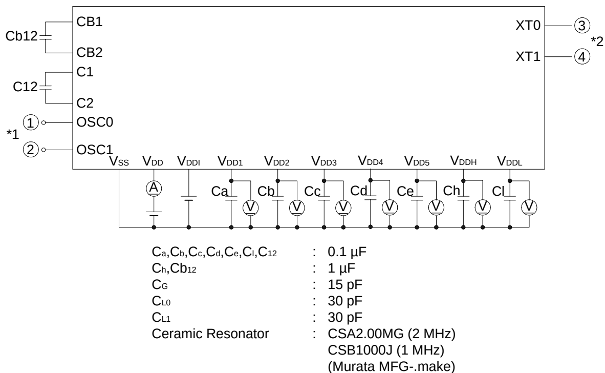
*1 RC Oscillator
