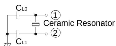
Ceramic Oscillator
