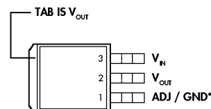
DD & DL PACKAGES (Top View)
