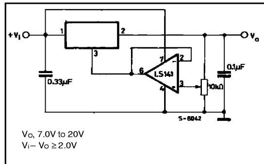
Figure 5 : Adjustable Output Regulator.
