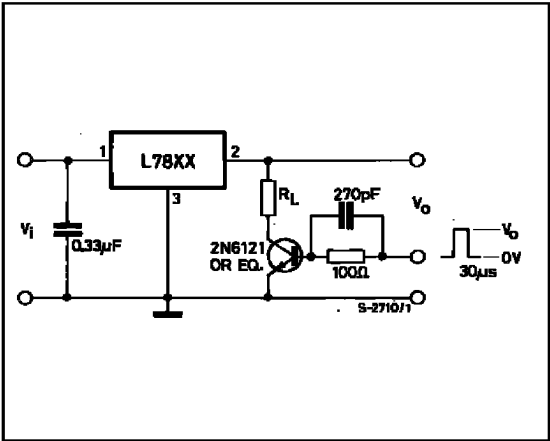
Figure 2 : Load Regulation.
