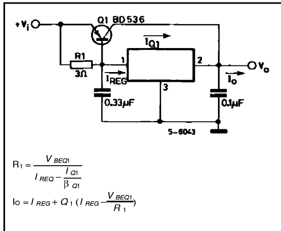
Figure 6 : Current Boost Regulator.
