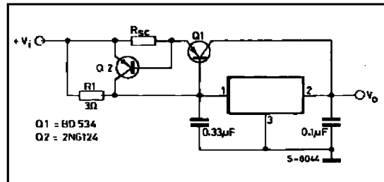
Figure 7 : Short-circuit Protection.
