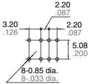
PC board pattern
