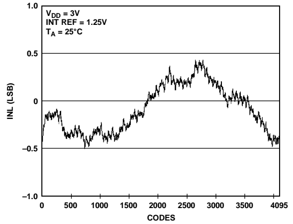
Figure 14. INL AD5629R-1—Internal Reference
