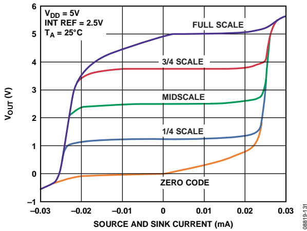
Figure 24. AD5669R-2 Source and Sink Capability
