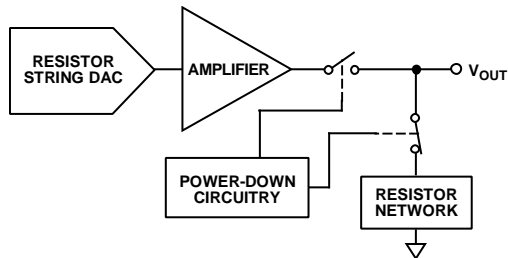
Figure 54. Output Stage During Power-Down
