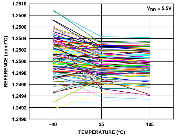
Figure 45. 1.25 V Reference Temperature Coefficient vs. Temperature
