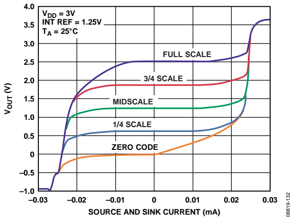
Figure 25. AD5669R-1 Source and Sink Capability
