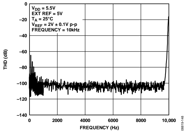
Figure 41. Total Harmonic Distortion
