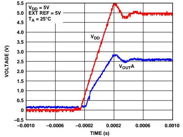
Figure 32. Power-On Reset to Midscale
