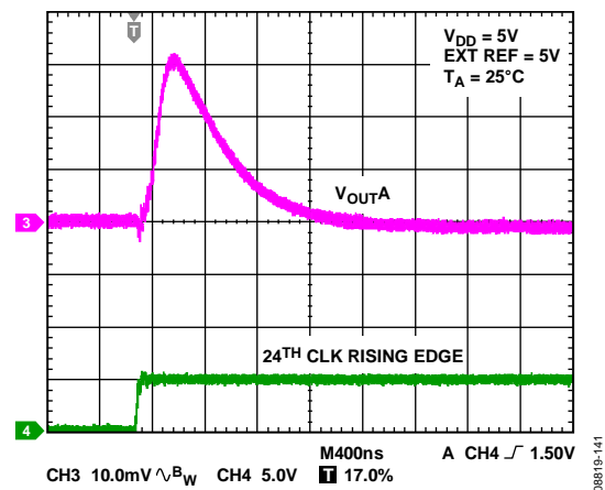
Figure 34. Digital-to-Analog Glitch Impulse (Negative)
