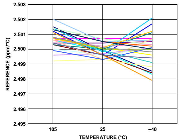
Figure 46. 2.5 V Reference Temperature Coefficient vs. Temperature
