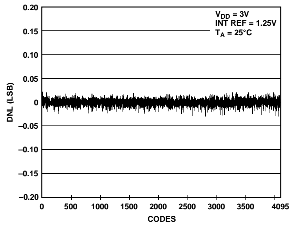
Figure 16. DNL AD5629R-1—Internal Reference
