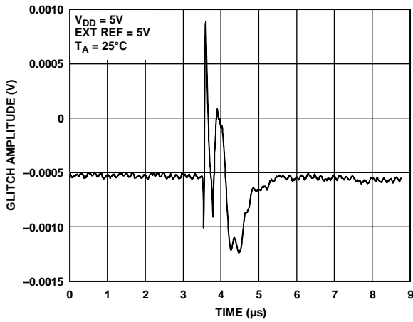
Figure 35. Analog Crosstalk
