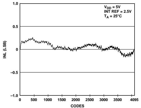
Figure 10. INL AD5629R-2—Internal Reference
