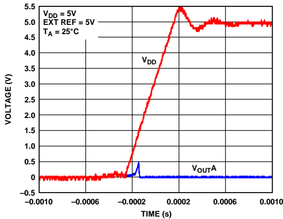
Figure 31. Power-On Reset to 0 V
