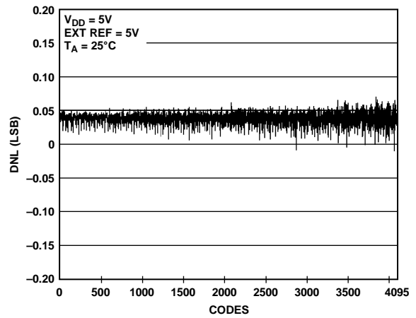
Figure 8. DNL AD5629R—External Reference
