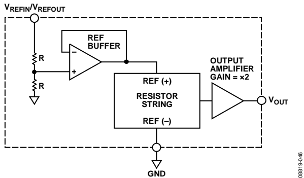
Figure 48. DAC Architecture for External Reference Configuration
