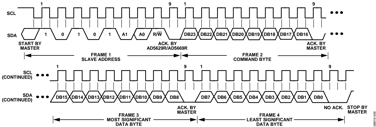
Figure 51. I 2 C Read Operation
