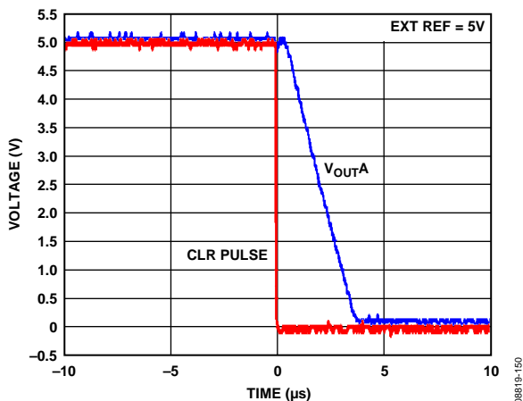
Figure 43. Hardware CLR
