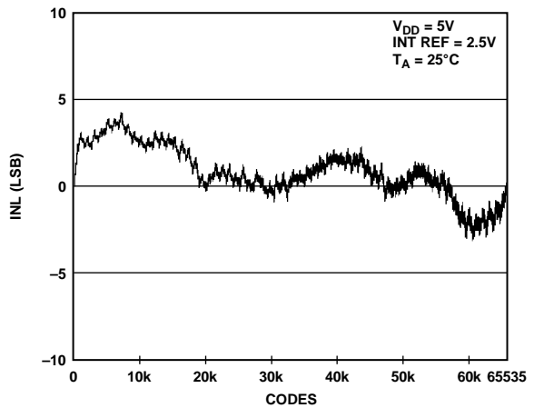
Figure 9. INL AD5669R-2—Internal Reference
