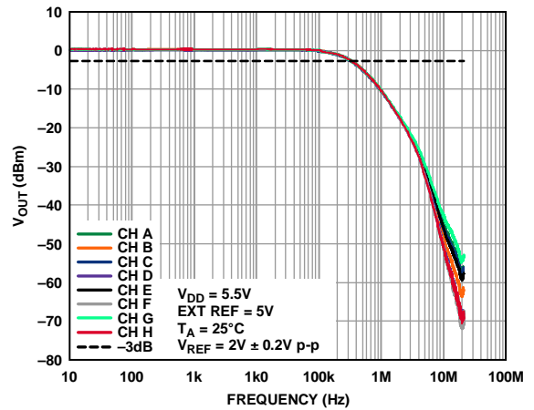
Figure 44. Multiplying Bandwidth
