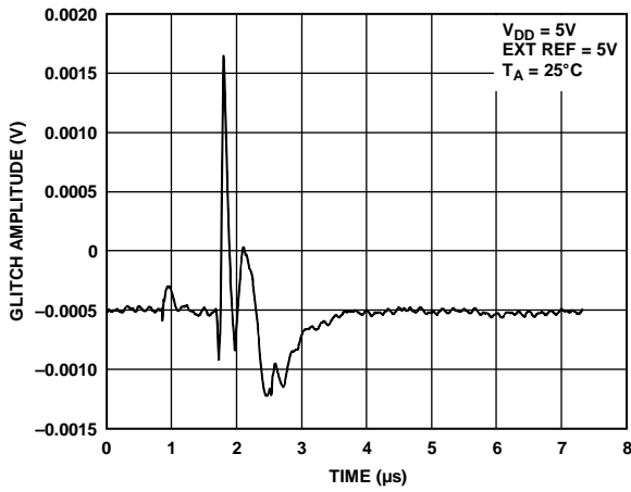
Figure 36. DAC-to-DAC Crosstalk
