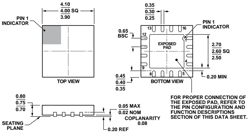
Figure 55. 16-Lead Lead Frame Chip Scale Package [LFCSP_WQ] 4 mm × 4 mm Body, Very Very Thin Quad (CP-16-17) Dimensions shown in millimeters
