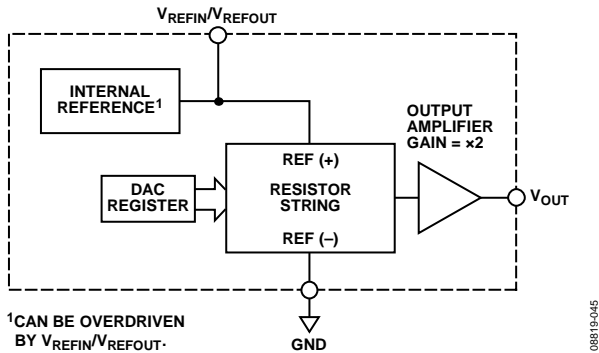
Figure 47. DAC Architecture for Internal Reference Configuration
