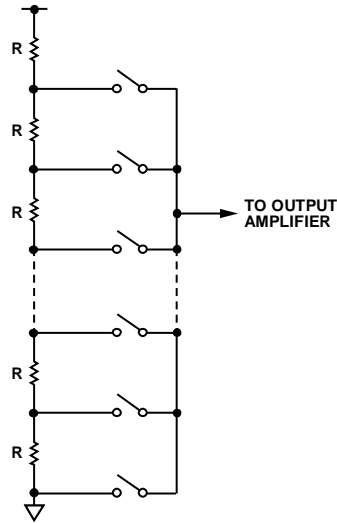
Figure 49. Resistor String
