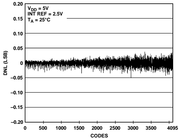
Figure 12. DNL AD5629R-2—Internal Reference
