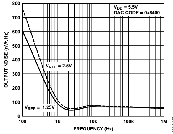
Figure 40. Noise Spectral Density, Internal Reference
