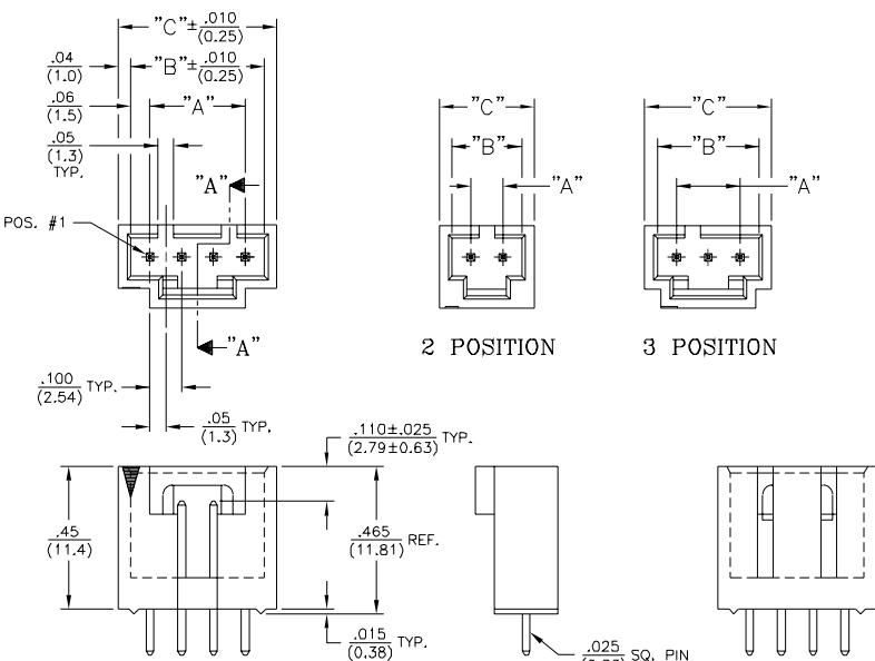
4 THRU 40 POSITION
