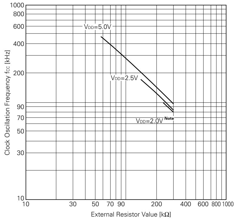
f_{cc} vs. R Characteristics Example (Reference Value) ( T_a=25^\circ\text{C} )
