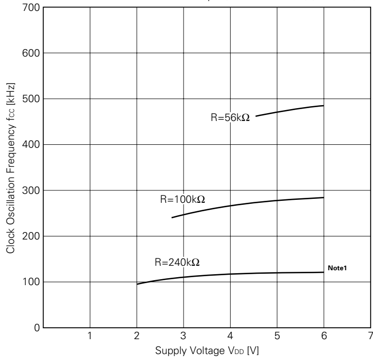
f_{cc} vs. V_{DD} Characteristics Example (Reference Value) ( T_a=25^\circ\text{C} )
