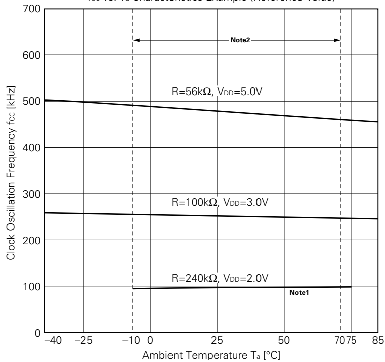
f_{cc} vs. T_a Characteristics Example (Reference Value)
