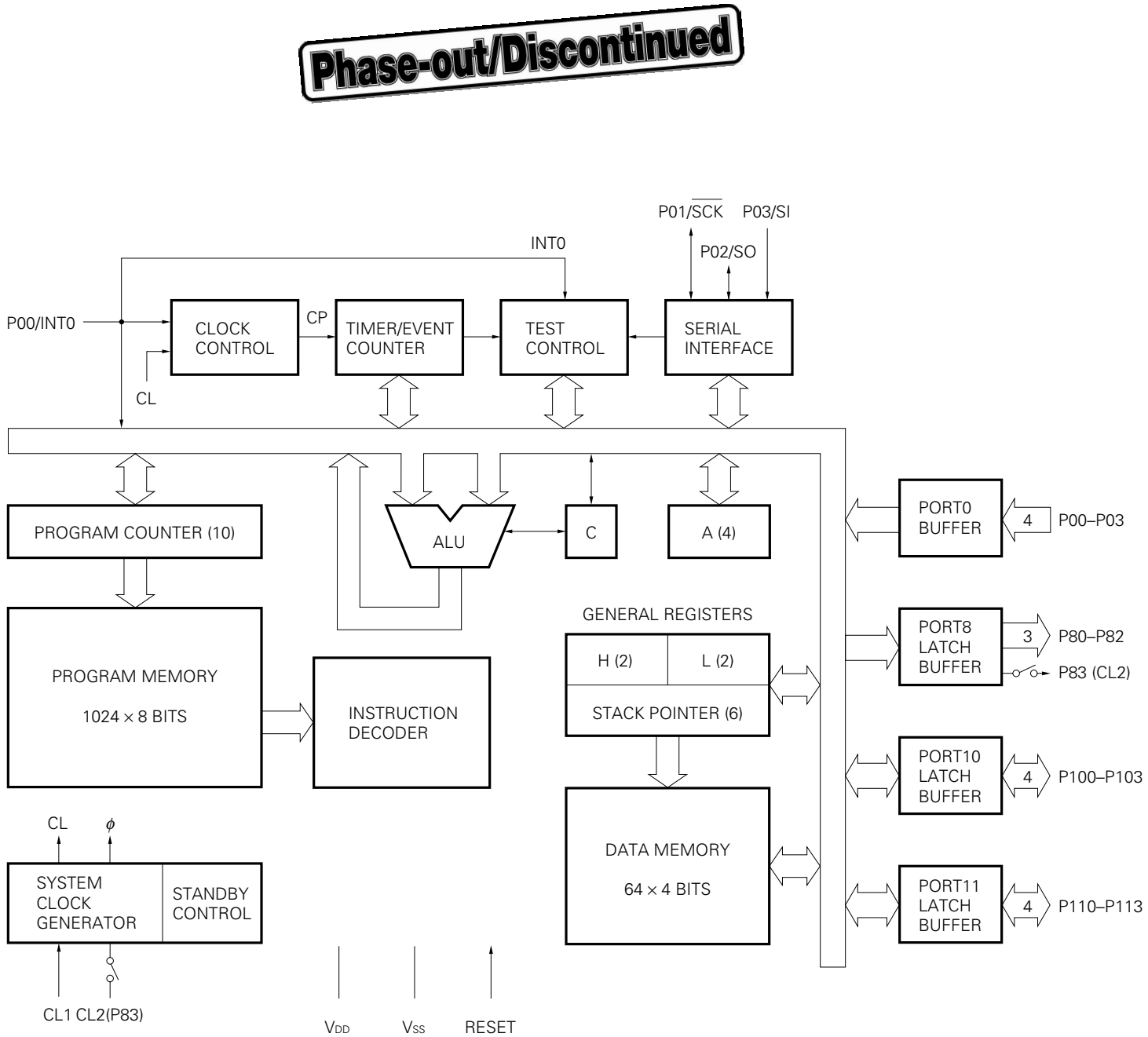
BLOCK DIAGRAM OF μPD7554A
