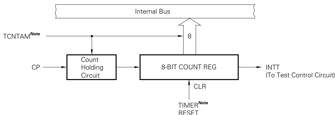
Fig. 2-12 Timer/Event Counter
