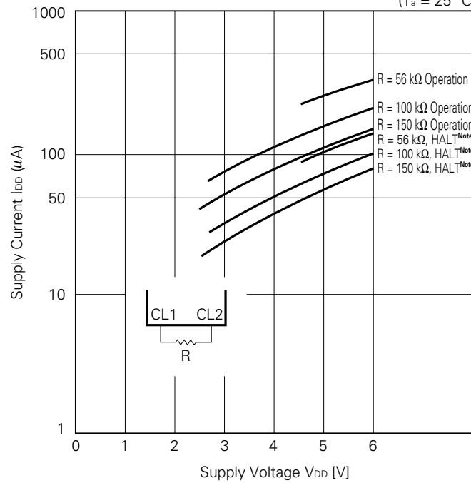
I_{DD} vs. V_{DD} Characteristic Example (Reference Value)
