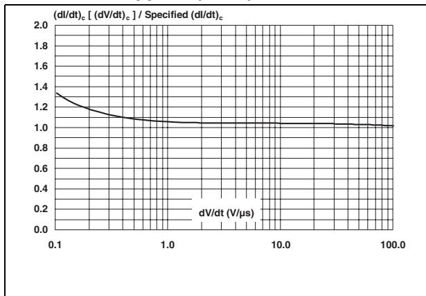
Figure 9. Relative variation of critical rate of decrease of main current (di/dt) c vs reapplied (dV/dt) c
