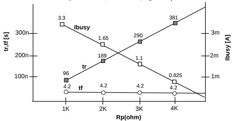
Fig 14 R_p vs t_r, t_f & R_p vs i_{busy}
