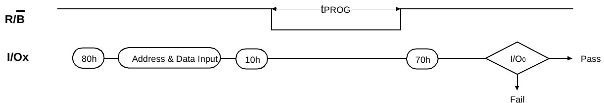
Figure 9. Program Operation
