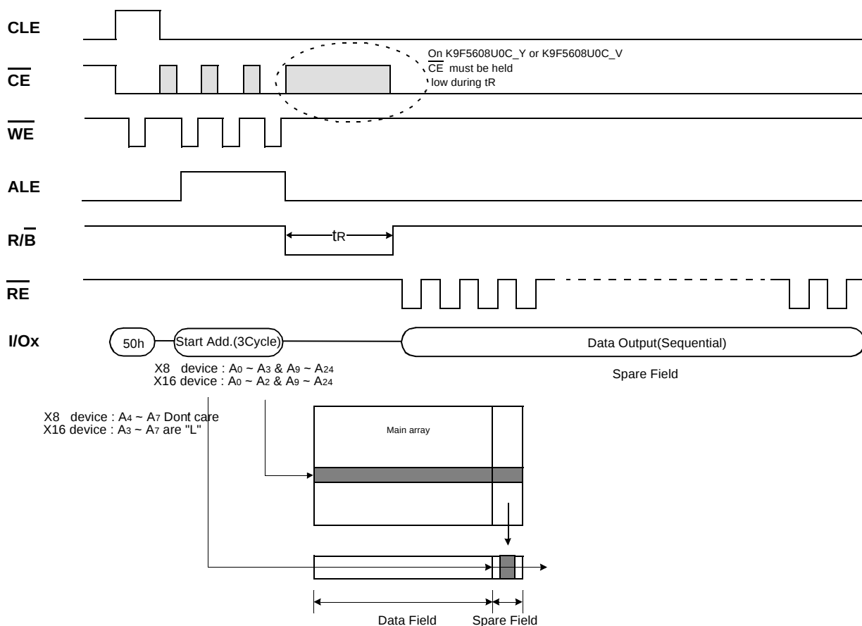
Figure 7-1. Sequential Row Read1 Operation (only for K9F5608U0C-Y or K9F5608U0C-V)
