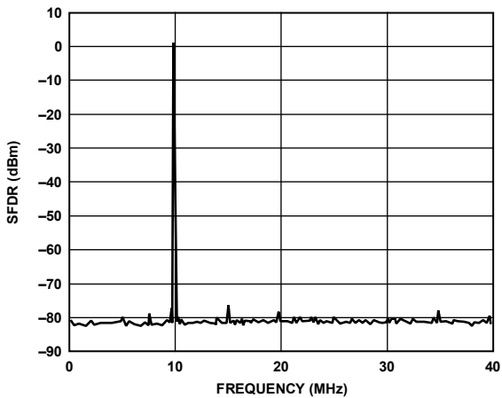
Figure 37. Single-Tone SFDR @ f_{CLK} = 125 MSPS
