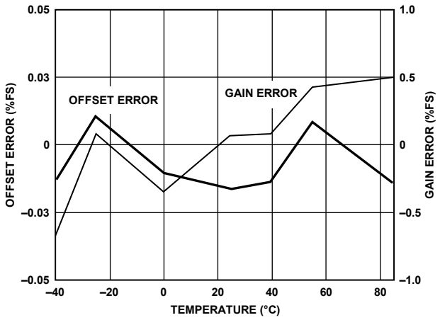
Figure 36. Gain and Offset Error vs. Temperature @ f_{CLK} = 125 MSPS
