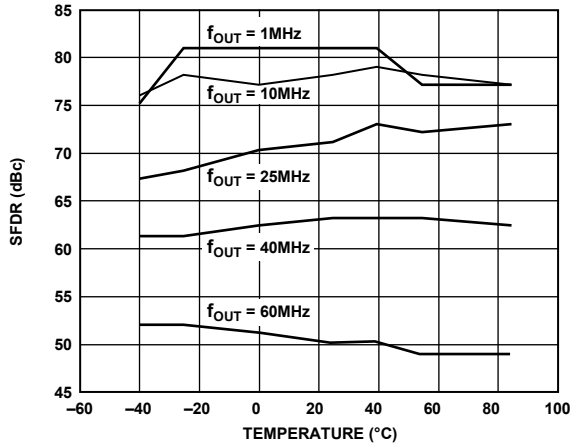
Figure 35. SFDR vs. Temperature @ 125 MSPS, 0 dBFS
