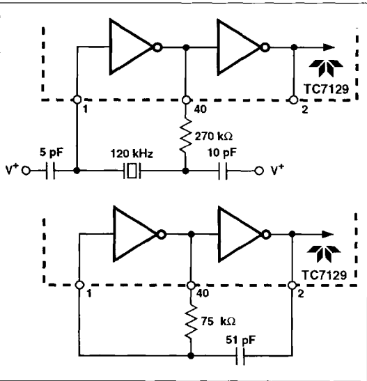
Figure 8 Oscillator Circuits
