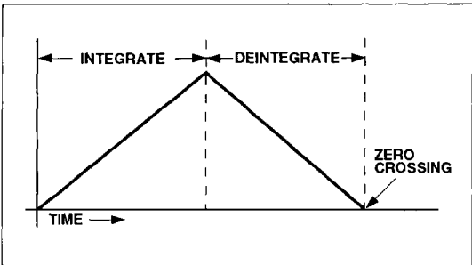
Figure 9 Dual-Slope Conversion
