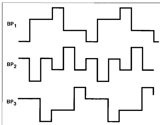
Figure 18 Backplane Waveforms
