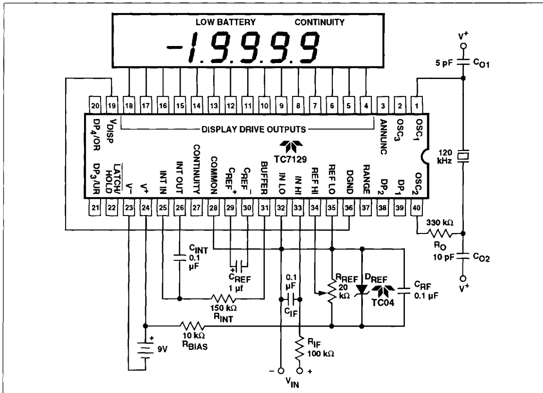
Figure 1 Standard Circuit
