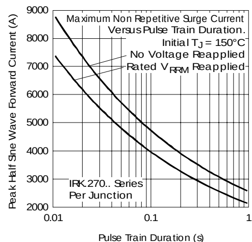
Fig. 20 - Maximum Non-Repetitive Surge Current
