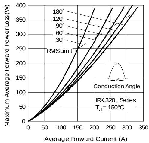
Fig. 25 - Forward Power Loss Characteristics
