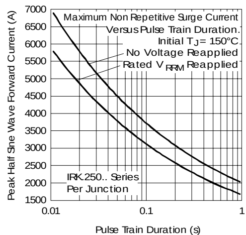
Fig. 9 - Maximum Non-Repetitive Surge Current
