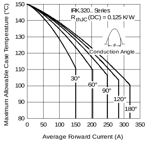
Fig. 23 - Current Ratings Characteristics
