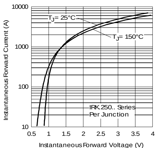
Fig. 10 - Forward Voltage Drop Characteristics
