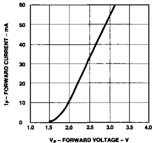
Figure 12. Forward Current vs. Forward Voltage.
