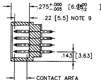
SECTION X-X
