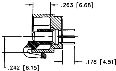
SECTION P-P (W/LOCATOR, SEE DETAIL P)
