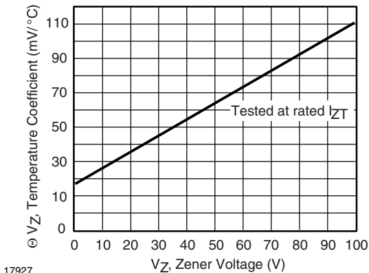
Fig. 3 - Typical Temperature Coefficients
