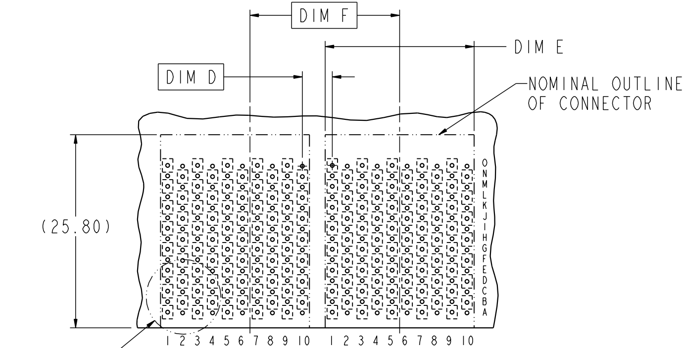
RECOMMENDED PCB LAYOUT FOR SINGLE ENDED APPLICATIONS COMPONENT SIDE (TWO ADJACENT FOOTPRINTS SHOWN)
