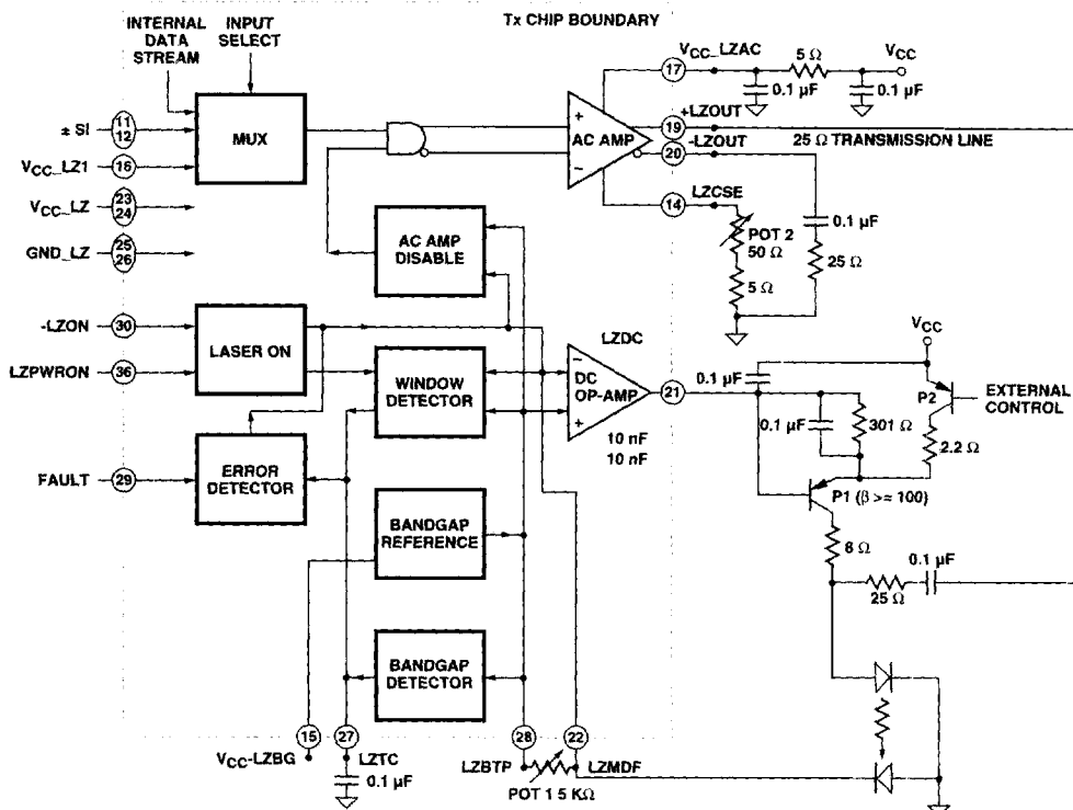
Figure 3. Laser Driver Block Diagram and External Circuitry.
