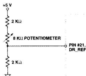
Figure 6. Simple Circuit Used to Adjust the Voltage on Rx pin # 21, DR_REF.
