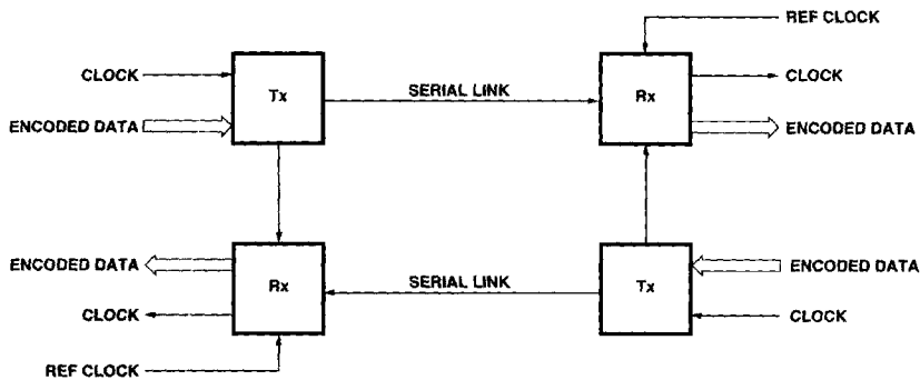
Figure 1. Point-to-Point Data Link.
