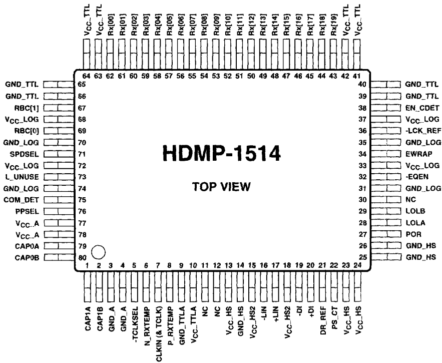
Figure 12. HDMP-1514 (Rx) Package Layout.
