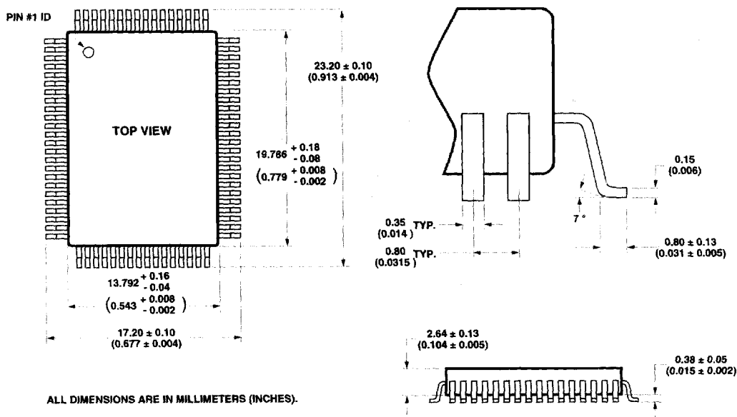
Figure 13. HDMP-1512 and HDMP-1514 Package Outline.
