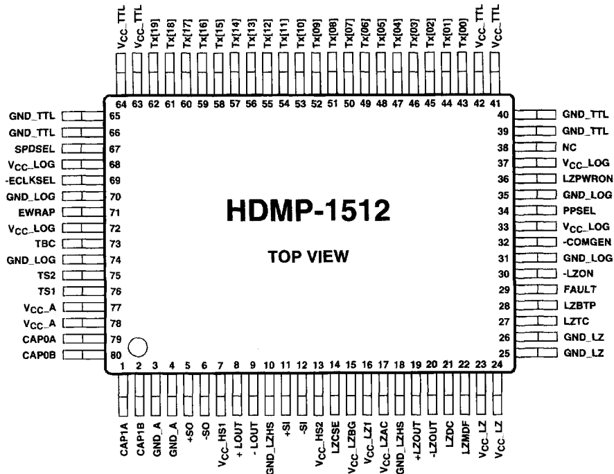
Figure 11. HDMP-1512 (Tx) Package Layout, Top View.
