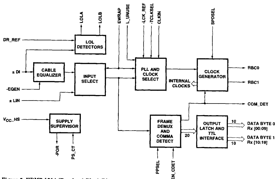
Figure 5. HDMP-1514 (Receiver) Block Diagram.
