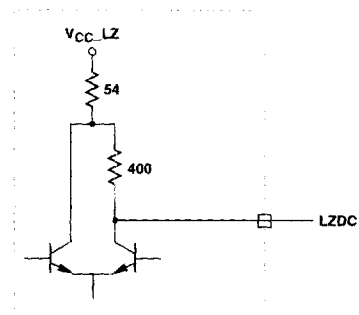
Figure 4. LZDC Equivalent Output Circuit (Tx pin # 21).
