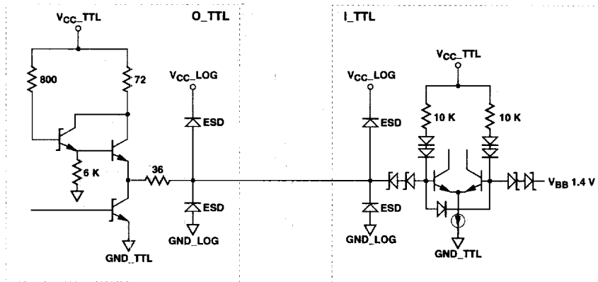
Figure 9. O-TTL and I-TTL Simplified Circuit Schematic.
