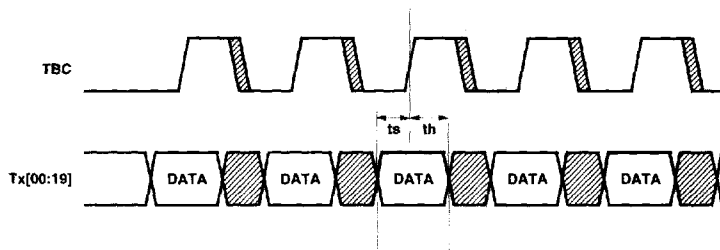
Figure 14. HDMP-1512 (Transmitter) Timing Diagram, with PPSEL = 0.
