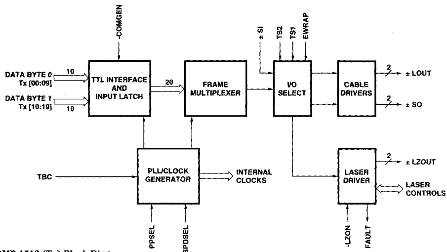
Figure 2. HDMP-1512 (Tx) Block Diagram.
