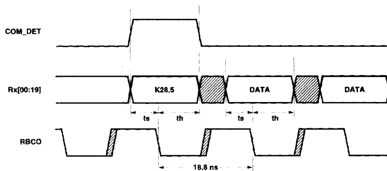
Figure 15. HDMP-1514 (Receiver) Timing Diagram, with PPSEL = 0.
