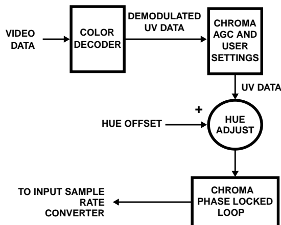
FIGURE 10. HUE ADJUST BLOCK DIAGRAM
