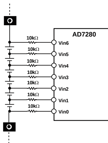
Figure 16. External Series Resistance
