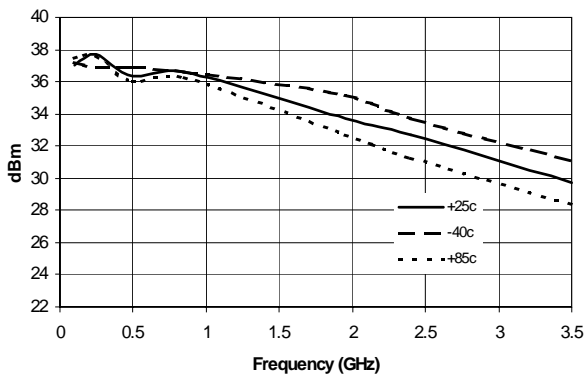
IP3 vs Frequency
