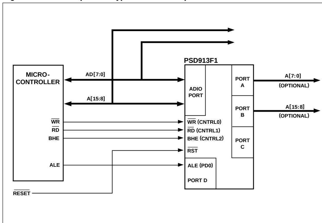
Figure 14. An Example of a Typical 8-Bit Multiplexed Bus Interface
