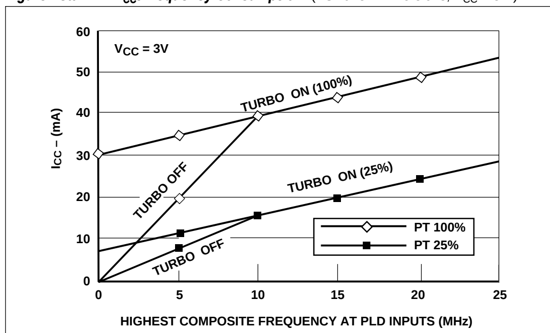
Figure 28a. PLD I_{CC} /Frequency Consumption (PSD913F1V Versions, V_{CC} = 3\text{ V} )
