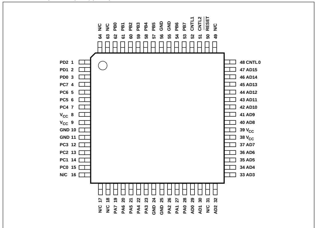
Figure 38. Drawing U4 – 64-Pin Plastic Thin Quad Flatpack (TQFP) (Package Type U)
