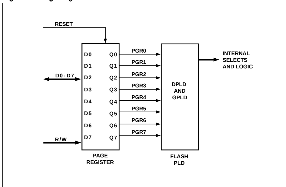
Figure 10. Page Register
