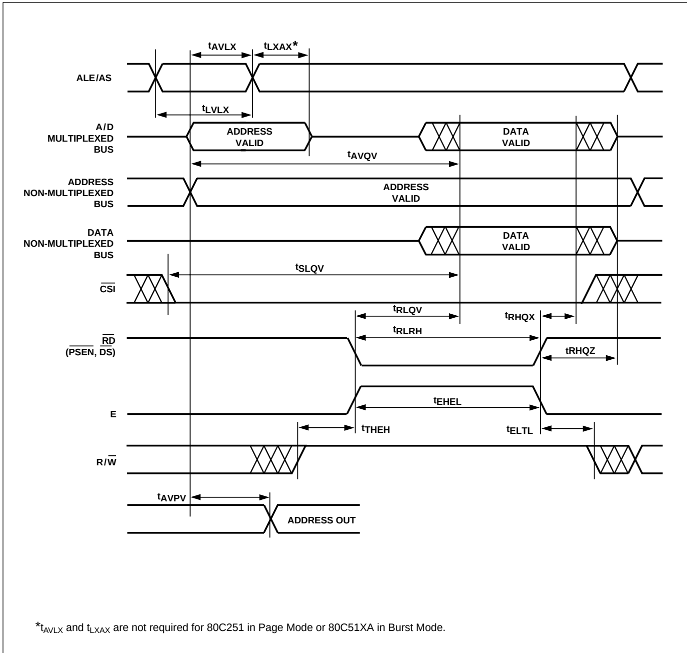
Figure 29. Read Timing
