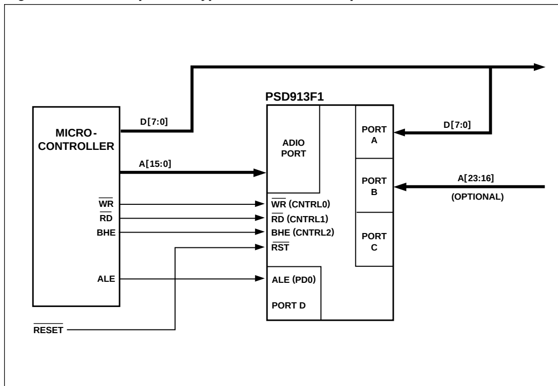
Figure 15. An Example of a Typical 8-Bit Non-Multiplexed Bus Interface
