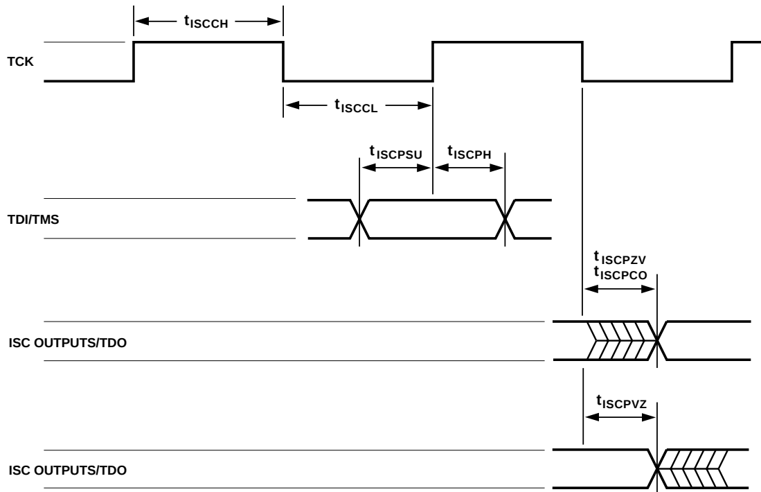
Figure 32. ISC Timing
