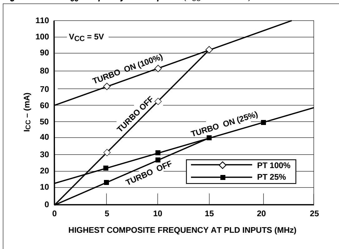
Figure 28. PLD I_{CC} /Frequency Consumption ( V_{CC} = 5\text{ V} \pm 10\% )
