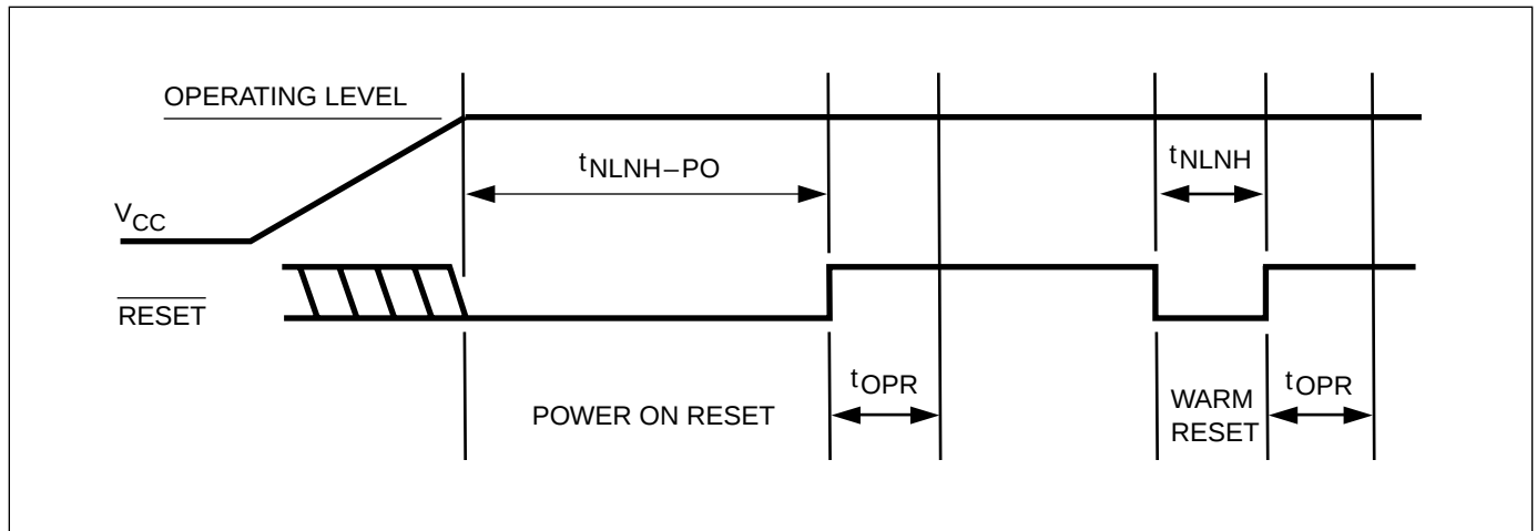
Figure 33. Reset Timing
