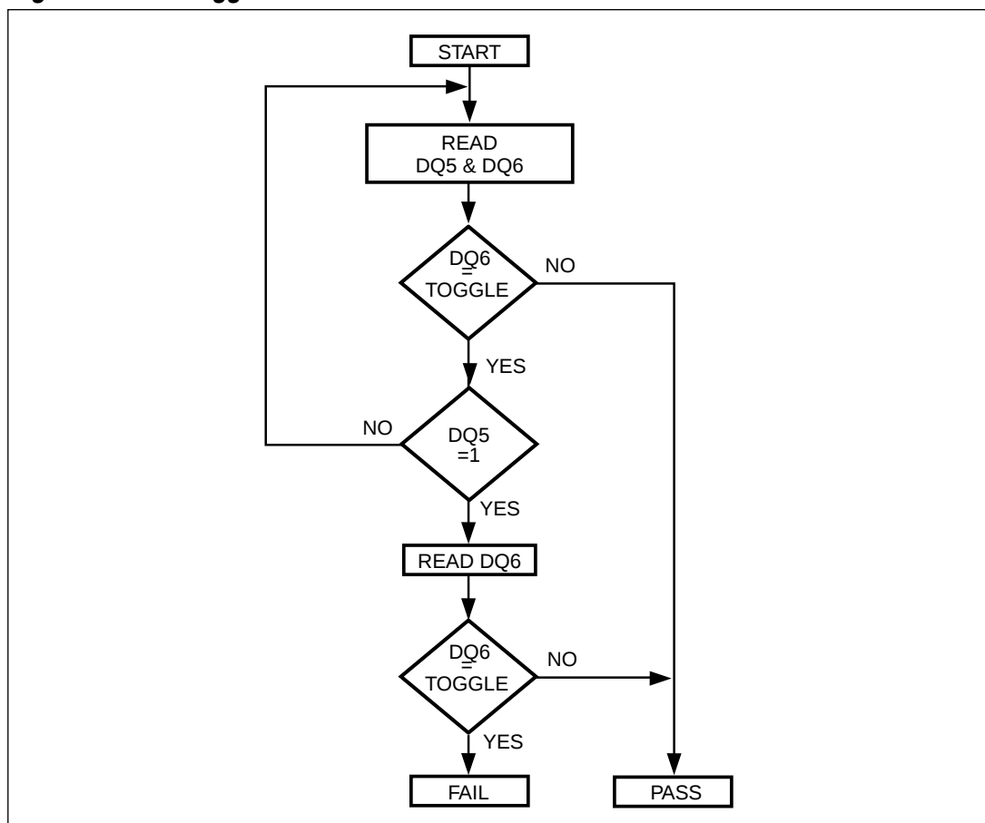
Figure 6. Data Toggle Flow Chart
