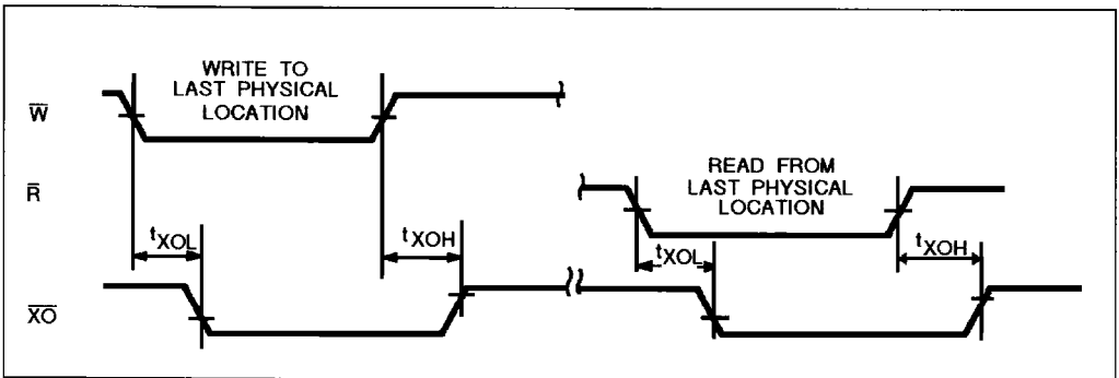
Figure 15 : Expansion Out.
