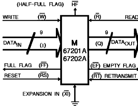
Figure 2 : Block Diagram of Single 512 x 9 and 1024 x 9.
