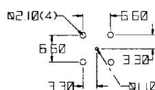
RECOMMENDED PCB LAYOUT (BOTTOM VIEW)
