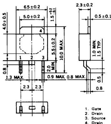
PACKAGE DIMENSIONS in millimeters
