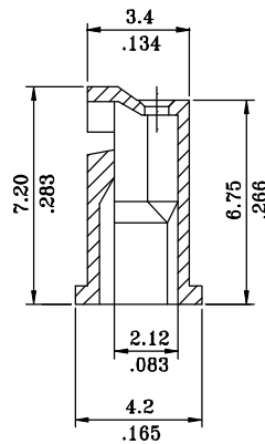
SECTION F-F
