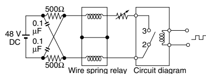
Circuit
