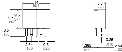
Self-clinching terminal
