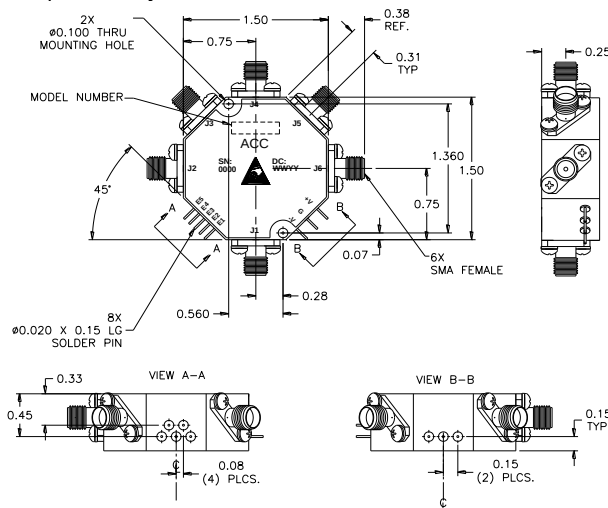
OUTLINE CASE STYLE S5
