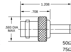
CABLE JACK TOOL CRIMP
