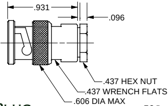
CABLE PLUG WRENCH CRIMP
