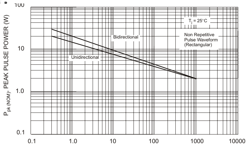
PULSE WIDTH (ms) Fig. 7 Pulse Rating Curve, P_{pk(NOM)} (W) vs. Pulse Width (ms)
