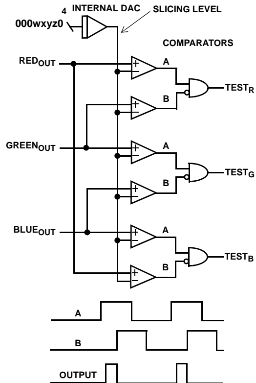
FIGURE 35. DELAY DETECTOR
