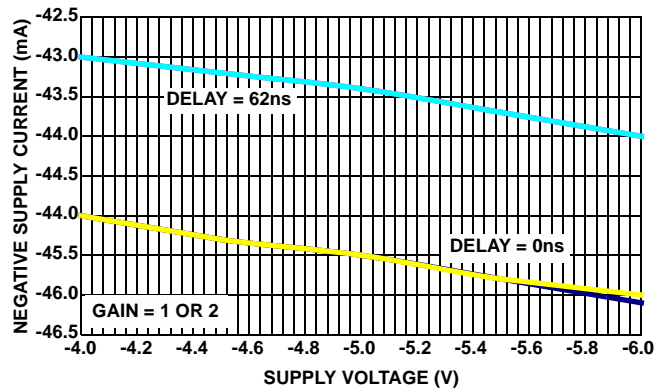
FIGURE 25. ISL59920 I_{SUPPLY-} vs V_{SPPLY-}
