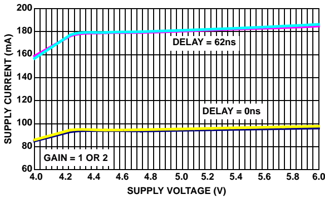
FIGURE 24. ISL59920 I_{SUPPLY+} vs V_{SPPLY+}
