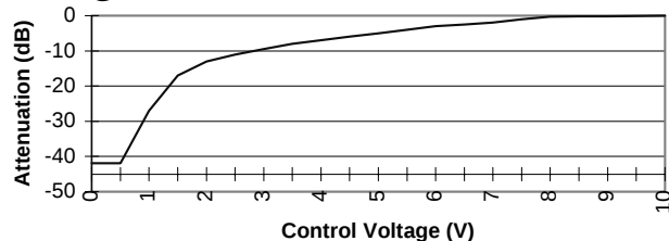
Attenuation vs Control Voltage @ 500 MHz
