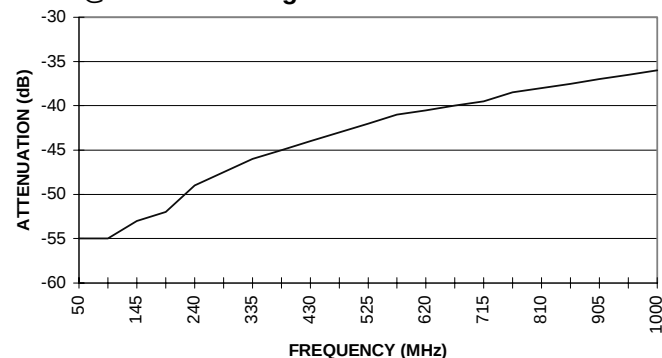
Attenuation vs Frequency @ Control Voltage = 0V
