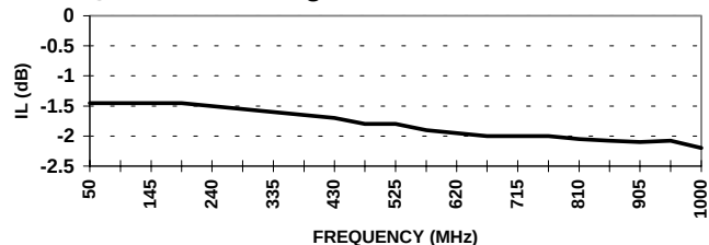
Insertion Loss vs Frequency @ Control Voltage = 10V
