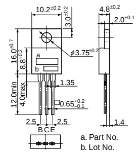
• No. 3 (TO-220)
