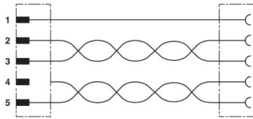
Circuit diagram
