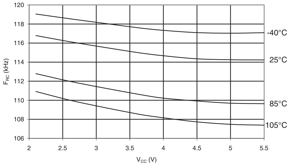
Figure 31-367. ATmega328P ^{\circ}C Watchdog Oscillator Frequency vs. V_{CC}
