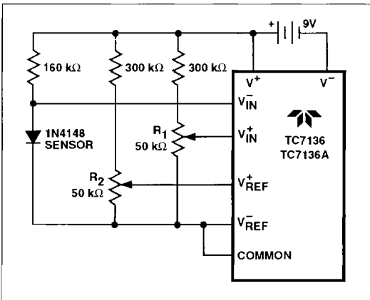
Figure 13 Temperature Sensor
