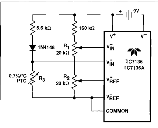
Figure 14 Positive Temperature Coefficient Resistor Temperature Sensor
