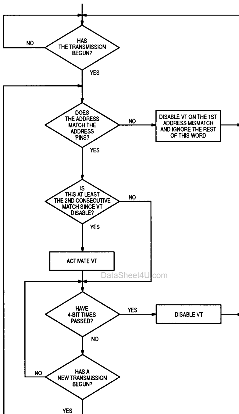
Figure 13. MC145028 Flowchart
