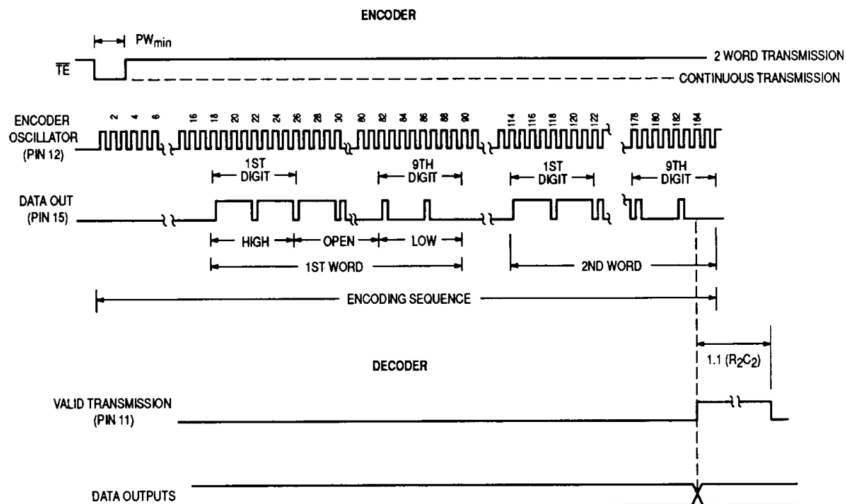
Figure 10. Timing Diagram
