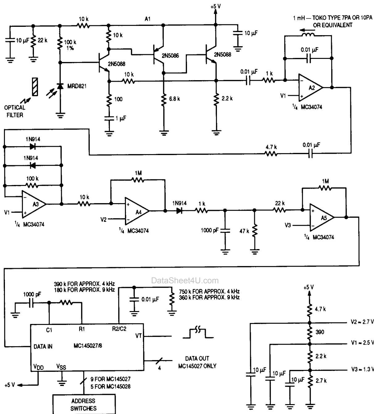
Figure 18. Infrared Receiver
