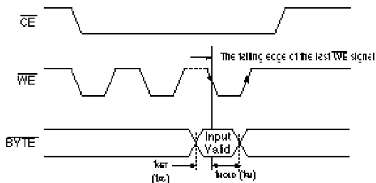
Timing Diagram for Write Operations
