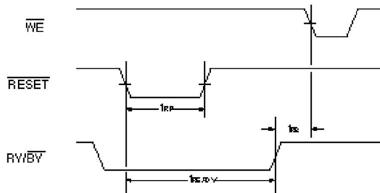
/RY/BY Timing Diagram
