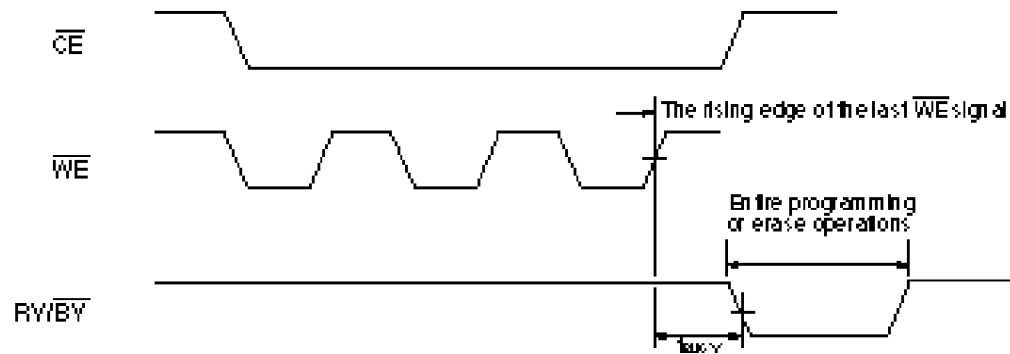
Timing Diagram during Program/Erase Operations
