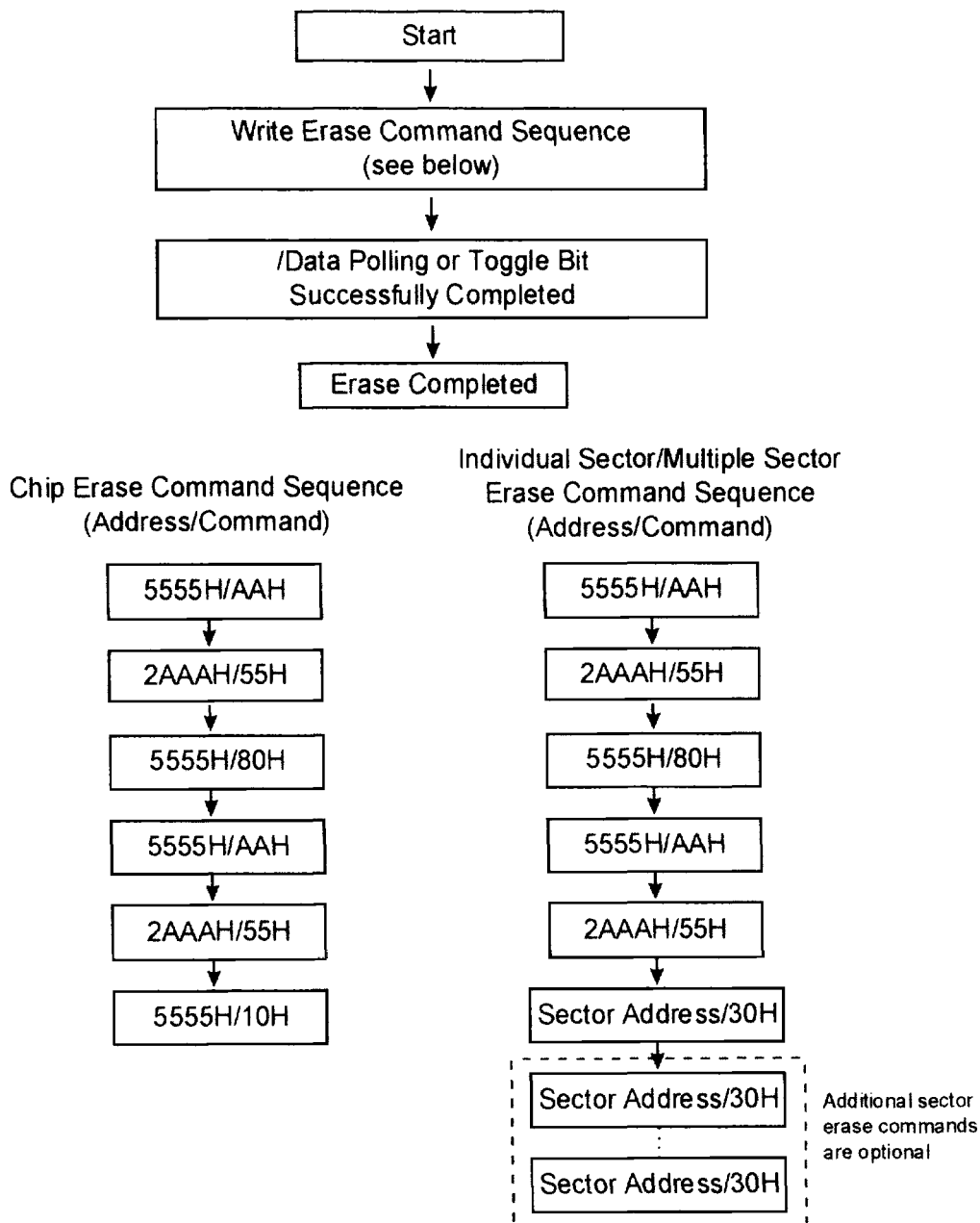
Figure 2. Internal Erase Algorithm
