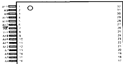
Standard TSOP
