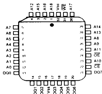
PLCC
