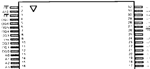
Reverse TSOP
