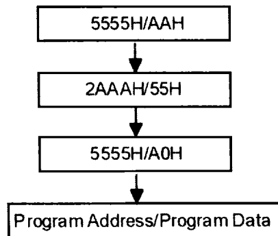
Program Command Sequence (Address/Command)
