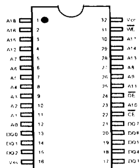
PDIP
