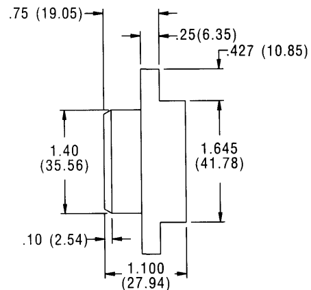
Socket side
