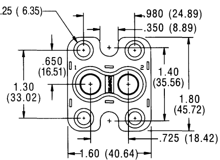
Front Views
