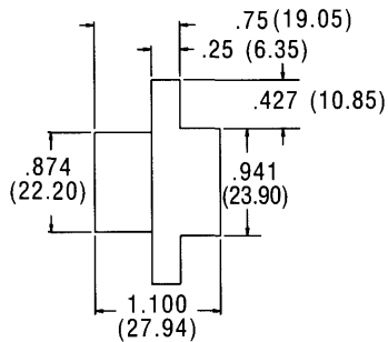
Pin side
