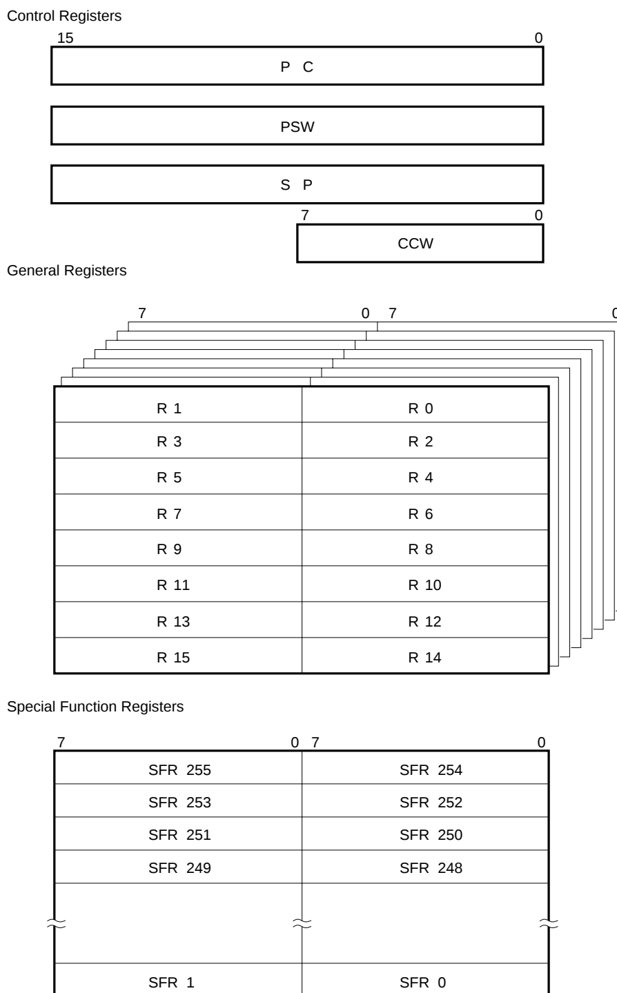
Figure 2-2. Register Configuration
