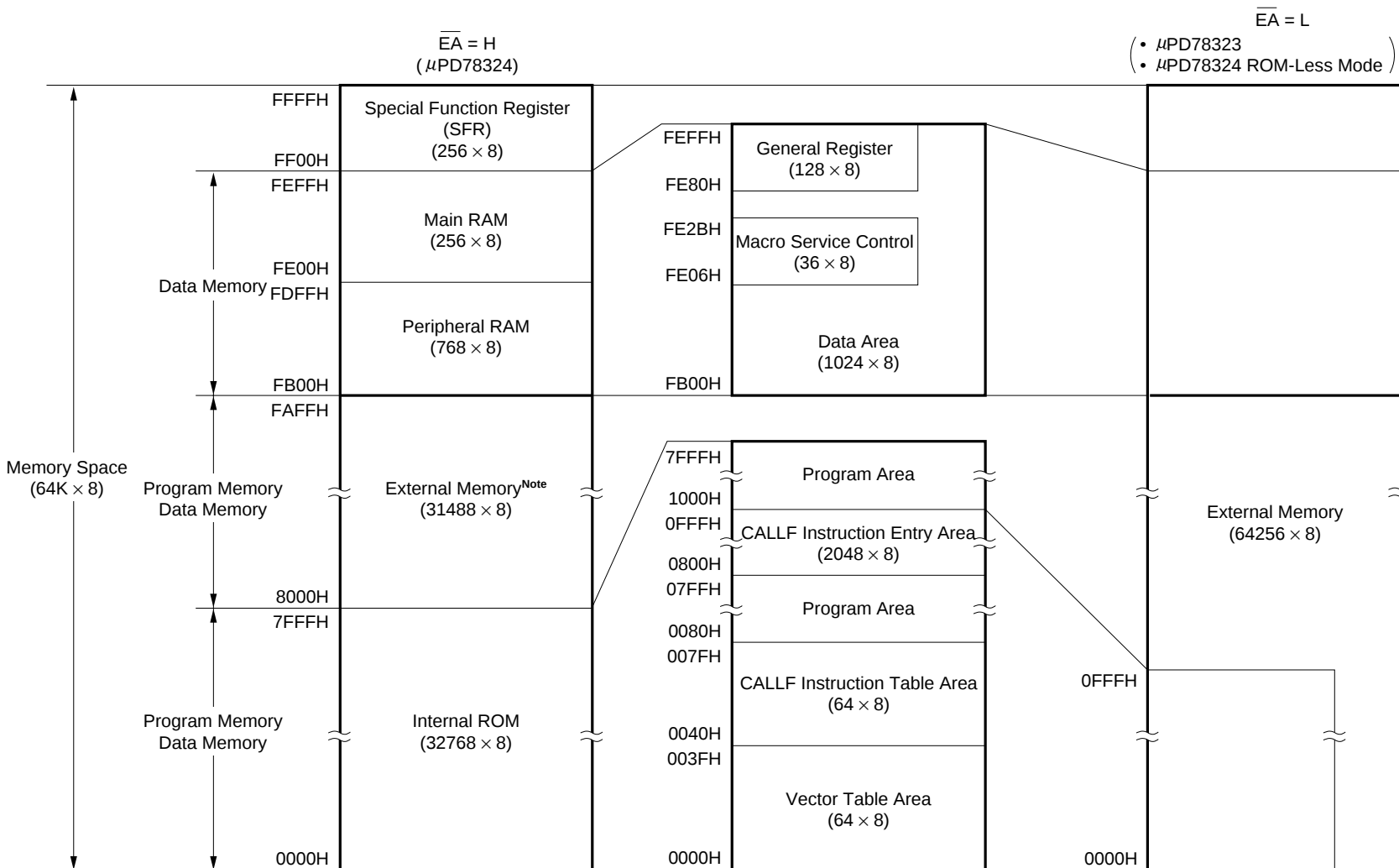
Figure 2-1. Memory Map
