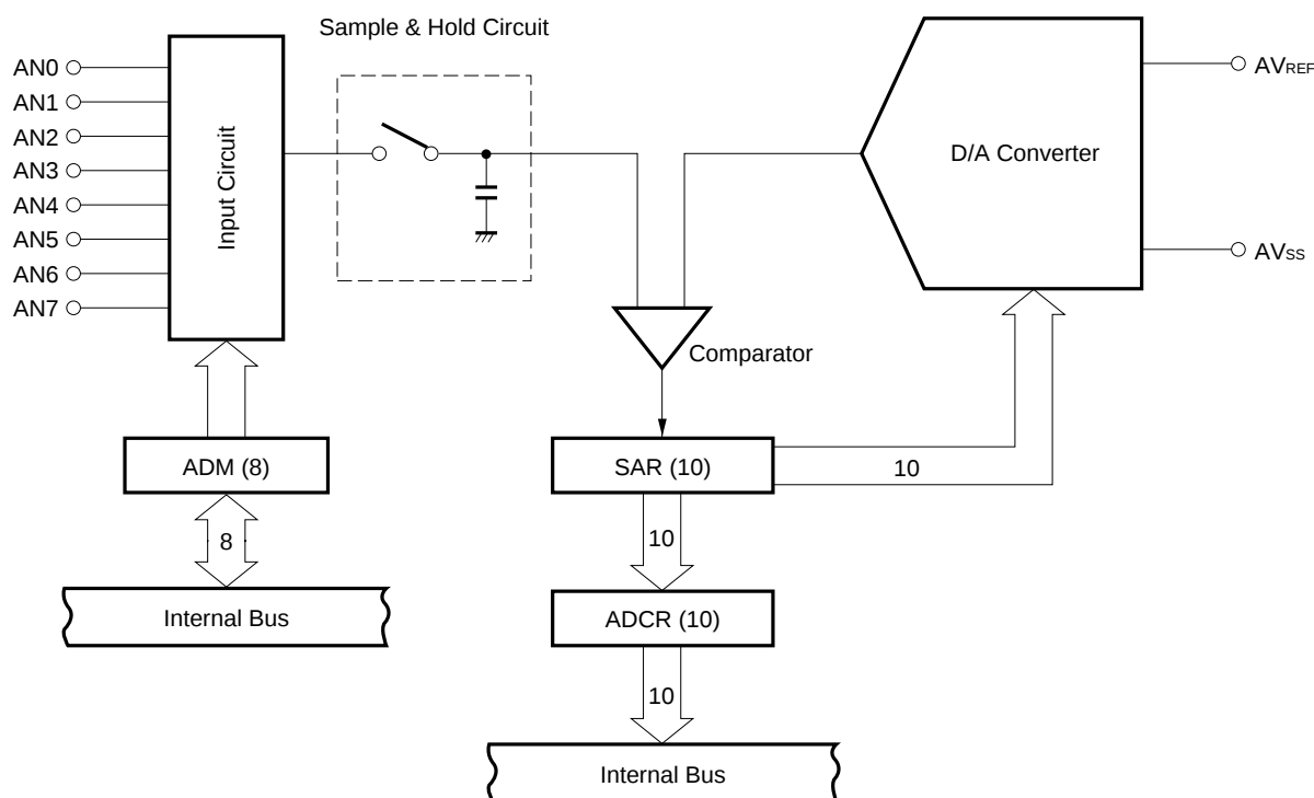
Figure 3-5. A/D Converter Block Diagram
