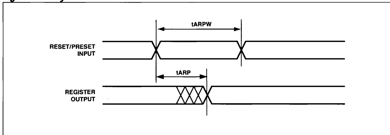
Figure 60. Asynchronous Reset/Preset
