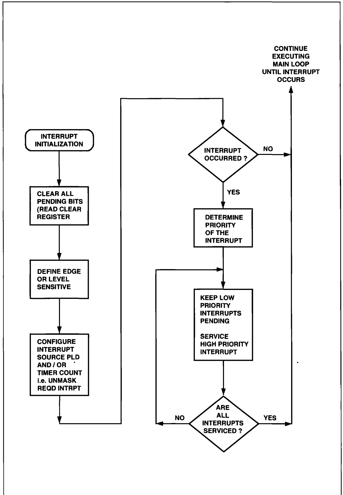
Figure 48. Interrupt Flowchart
