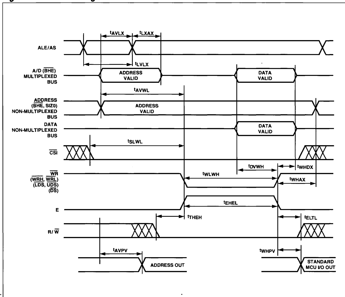
Figure 53. Write Timing
