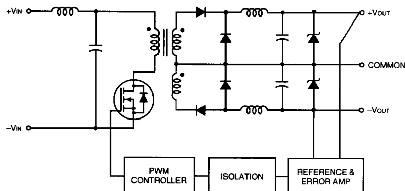
Figure 1. Simplified Schematic
