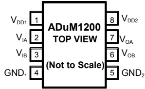
Figure 4. DuM1200 Pin Configuration
