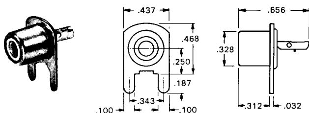
Mounting Detail
