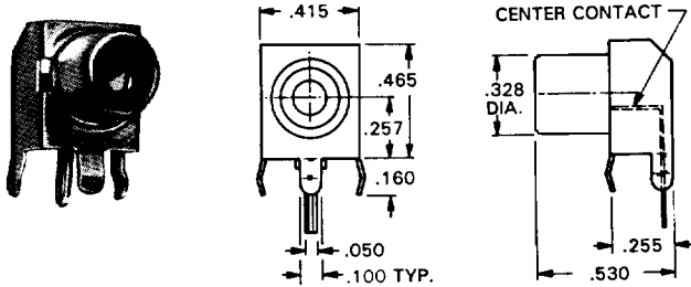
Mounting Detail
