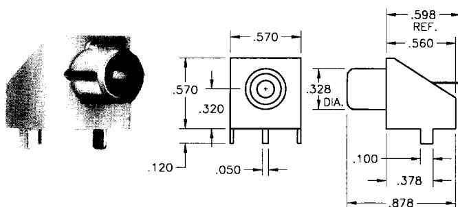
Mounting Detail
