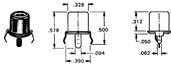
Mounting Detail
