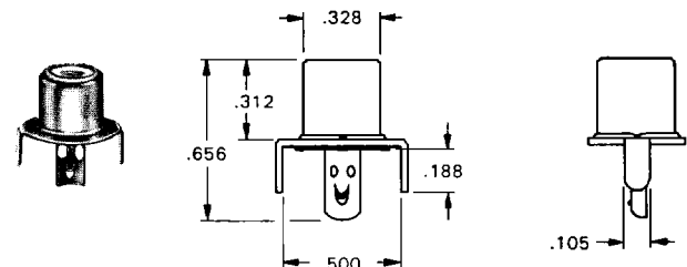
Mounting Detail
