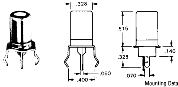
Mounting Detail
