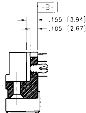
SECTION W-W
