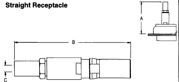
Crimp/Clamp
