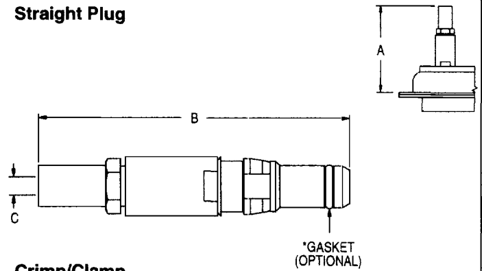
Crimp/Clamp
