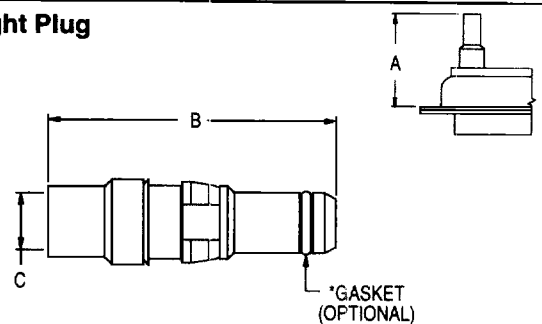
Direct Solder
