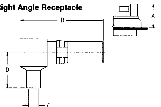
Direct Solder
