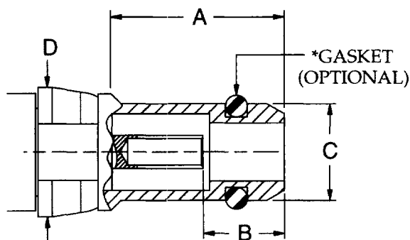
PLUG
