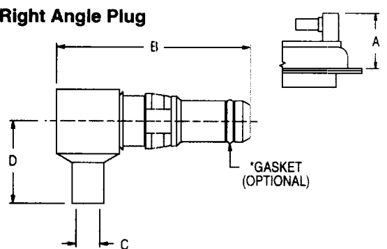
Direct Solder
