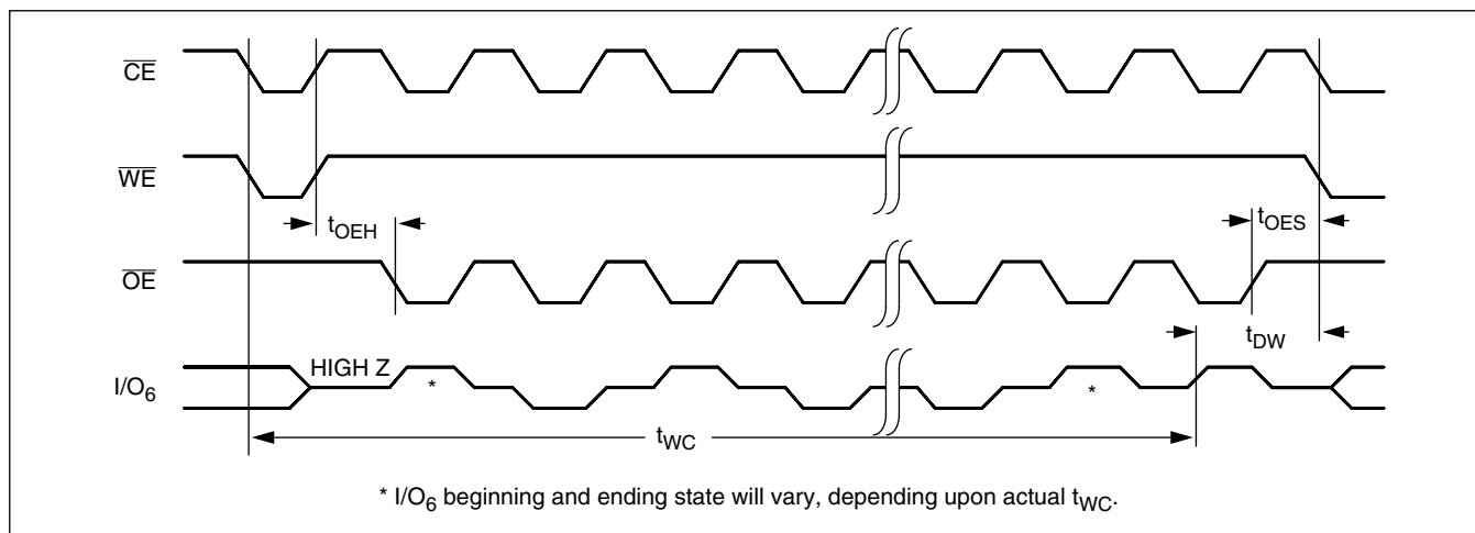
Toggle Bit Timing Diagram (11)
