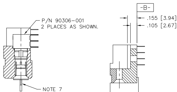
SECTION P-P
