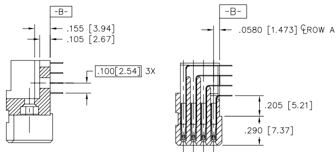
SECTION X-X
