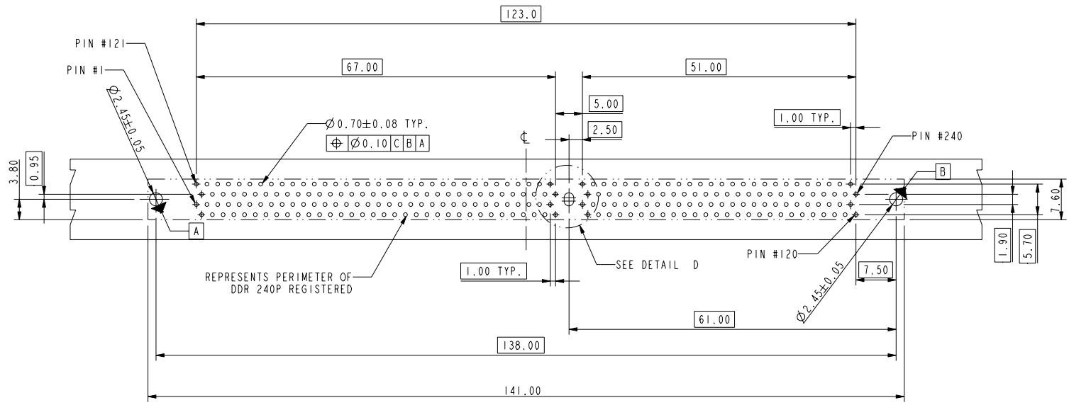
RECOMMENDED CIRCUIT BOARD HOLE LAYOUT SCALE 1.000
